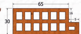
WPC Offset Window Profile
