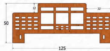
WPC Double Rebate Door & Window Frame
