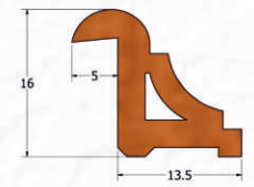
WPC Glass Fixing Strip
