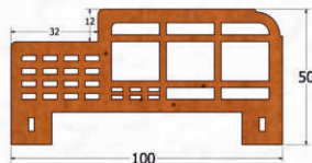
WPC Single Rebate Door & Window Frame
