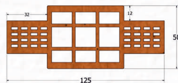
WPC Four Rebate Window Frame
