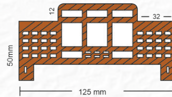
WPC DOUBLE REBATE DOOR & WINDOW FRAME
