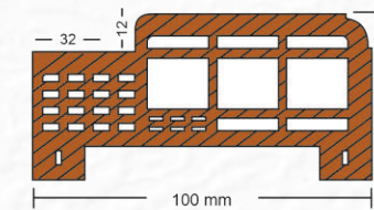
WPC SINGLE REBATE DOOR & WINDOW FRAME
